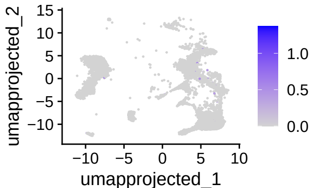
CYP7B1
