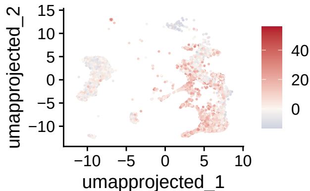
Factor_9_score
