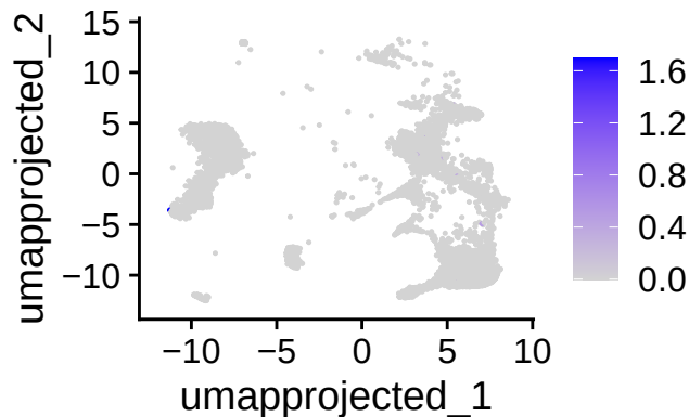
Factor_9_score
