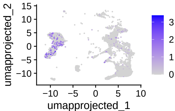
CYP7B1
