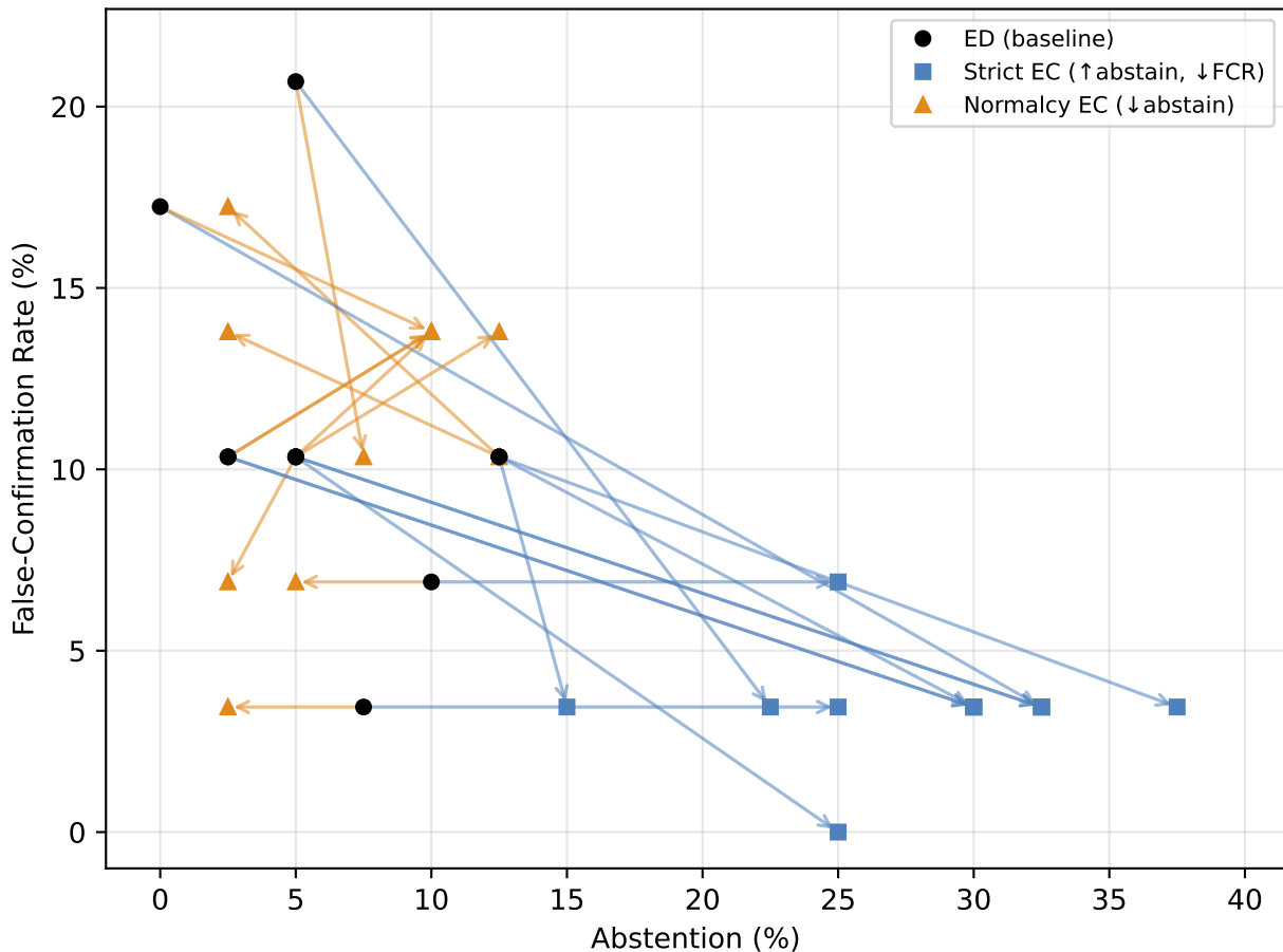
The Hydraulic Effect: conserved commitment-abstention trade-off (12 models)
