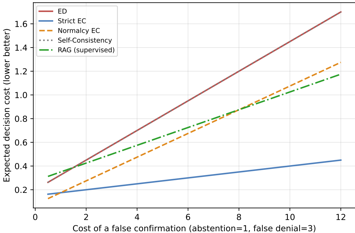
Cost-sensitive operating point (gpt-5.5): Strict EC wins as FC cost rises
