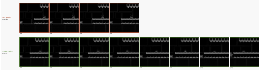
Figure 3: Decoded visual continuation from a real gameplay prefix. The first four frames are recorded Sobel observations; the remaining frames are sampled autoregressively from the V7 world model under the recorded future action sequence and decoded through the FSQ decoder.
