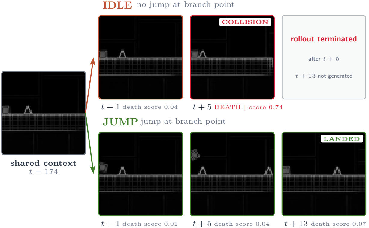
Figure 2 Action-conditioning diagnostic from one shared four-frame context. The rows are aligned at t + 1 and t + 5 : changing only the first future action makes the idle branch collide and terminate, while the jump branch clears the spike and lands by t + 13 .
