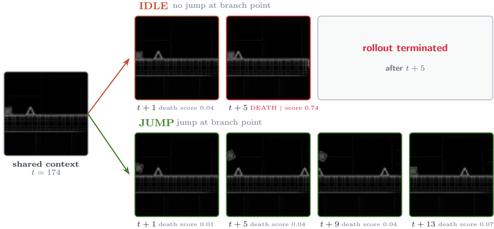
Figure 2 Greedy continuations from one reconstructed four-frame prefix; only the first future action differs. At t+1, t+5, t+9, t+13 , the jump branch clears the spike. The idle branch terminates at t+5 (death score 0.74), so later frames are not generated.
