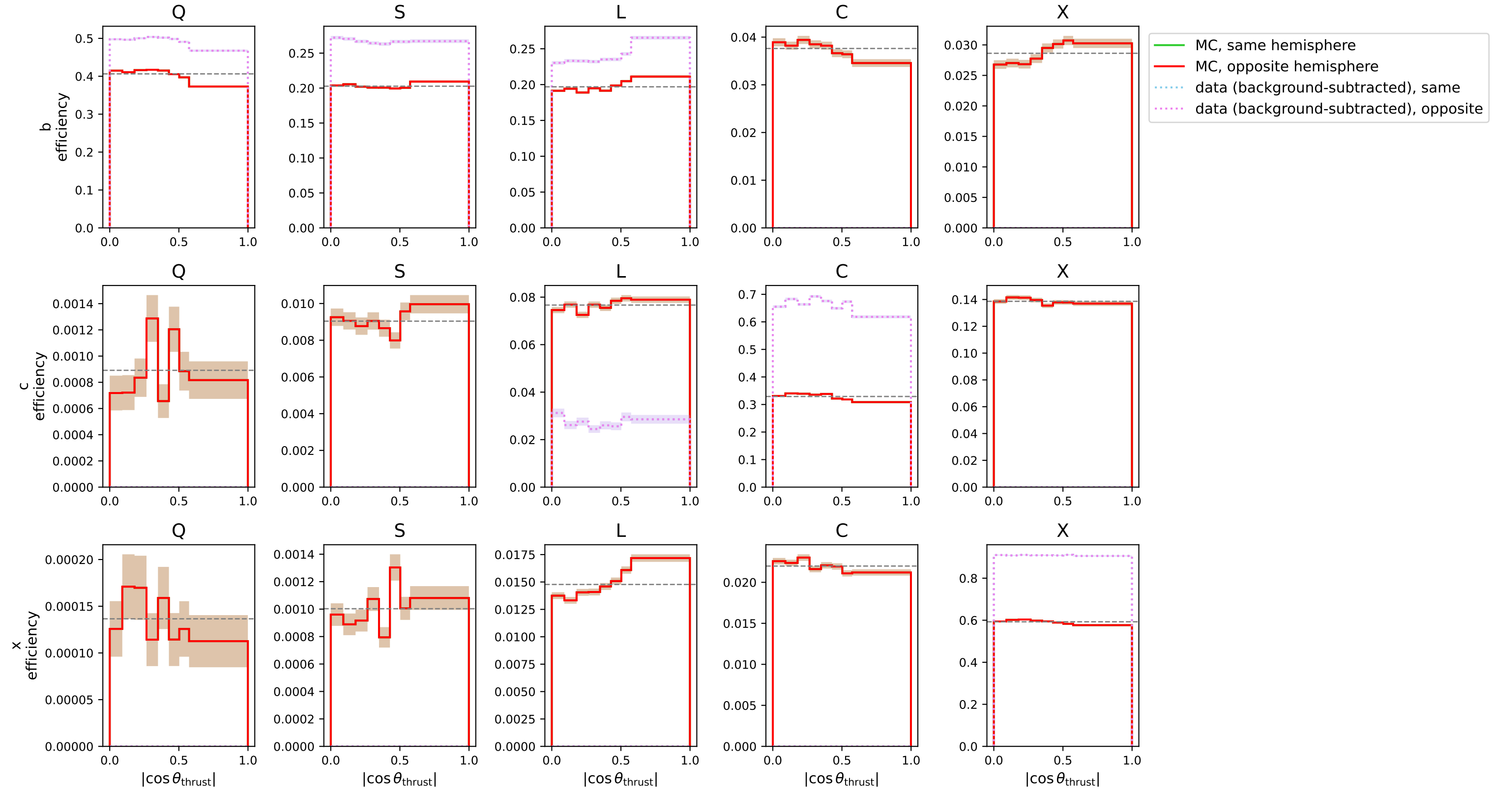
Same vs. opposite hemisphere efficiency vs. \cos\theta_{\text{thrust}}
