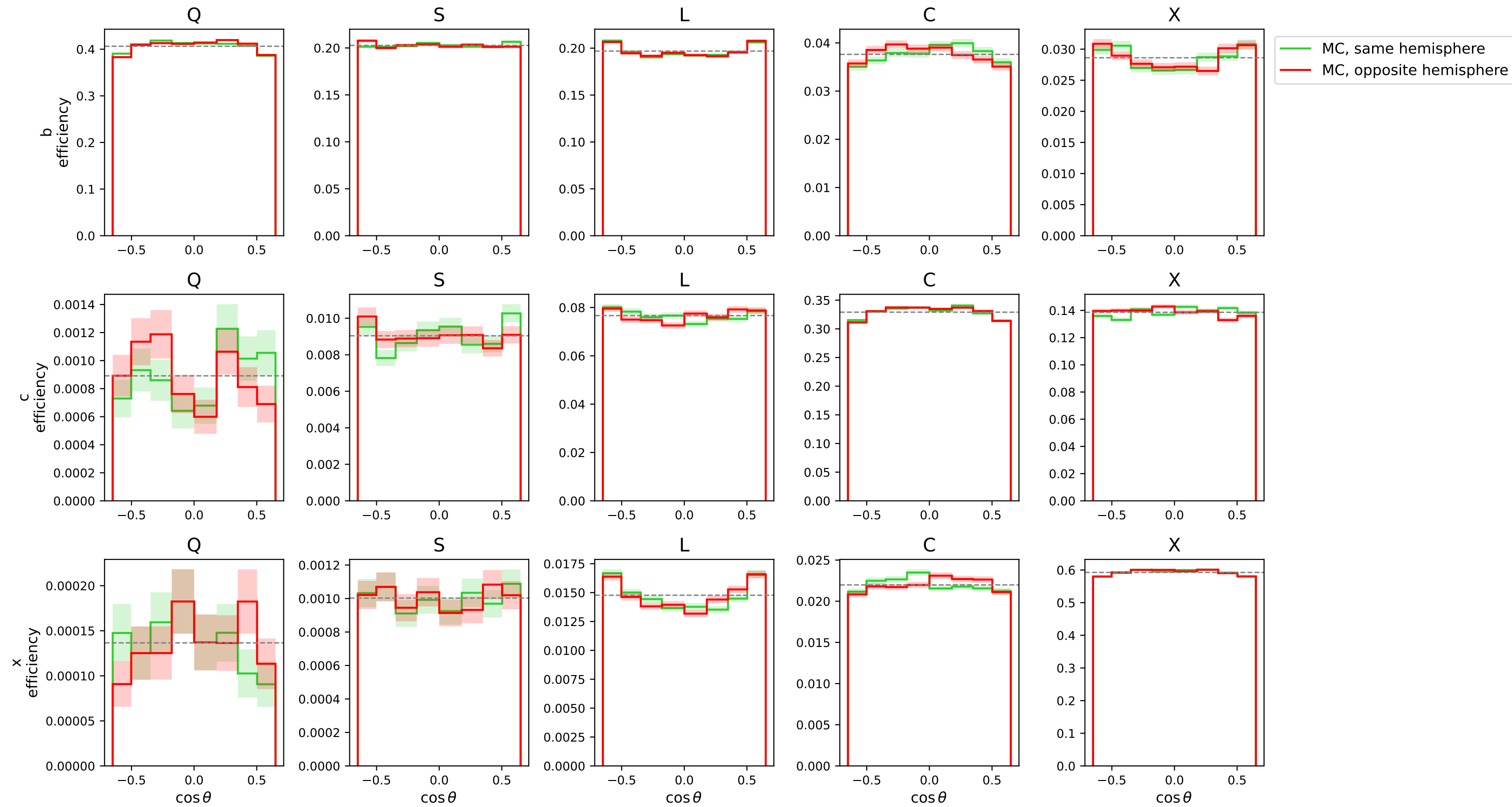
Same vs. opposite hemisphere efficiency vs. \cos\theta (simulation only)
