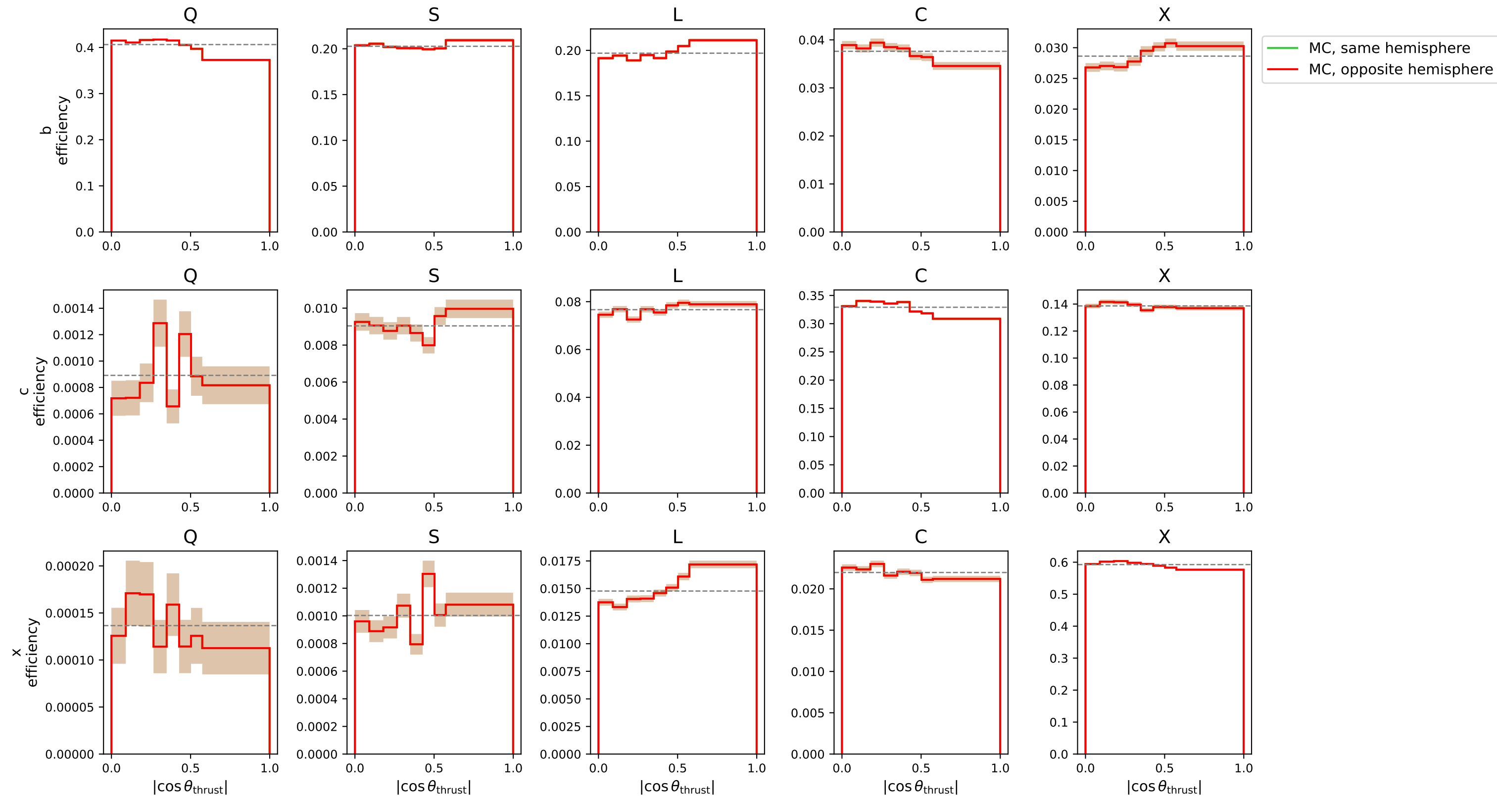
Same vs. opposite hemisphere efficiency vs. \cos\theta_{\text{thrust}} (simulation only)
