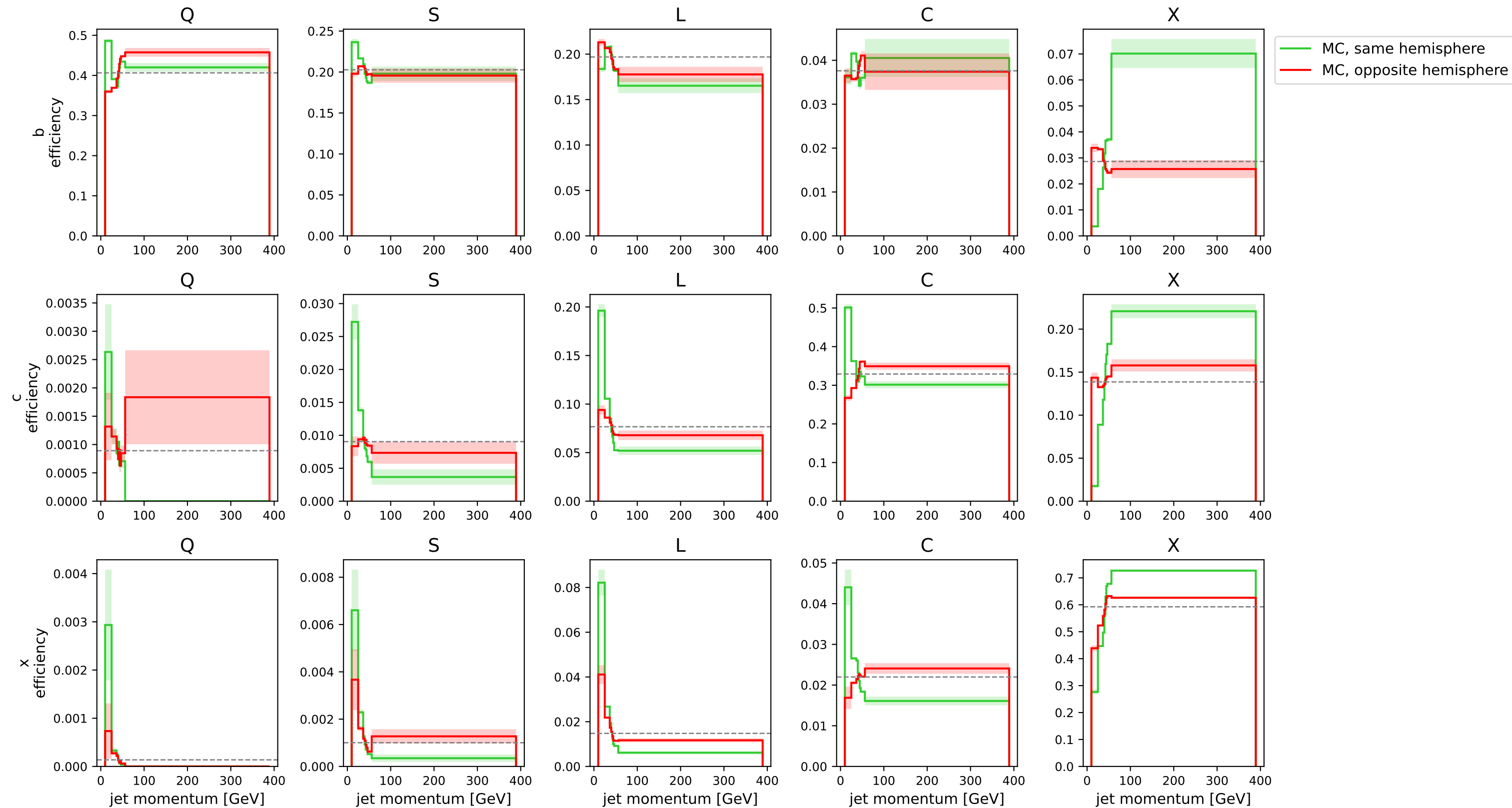
Same vs. opposite hemisphere efficiency vs. jet_momentum (simulation only)
