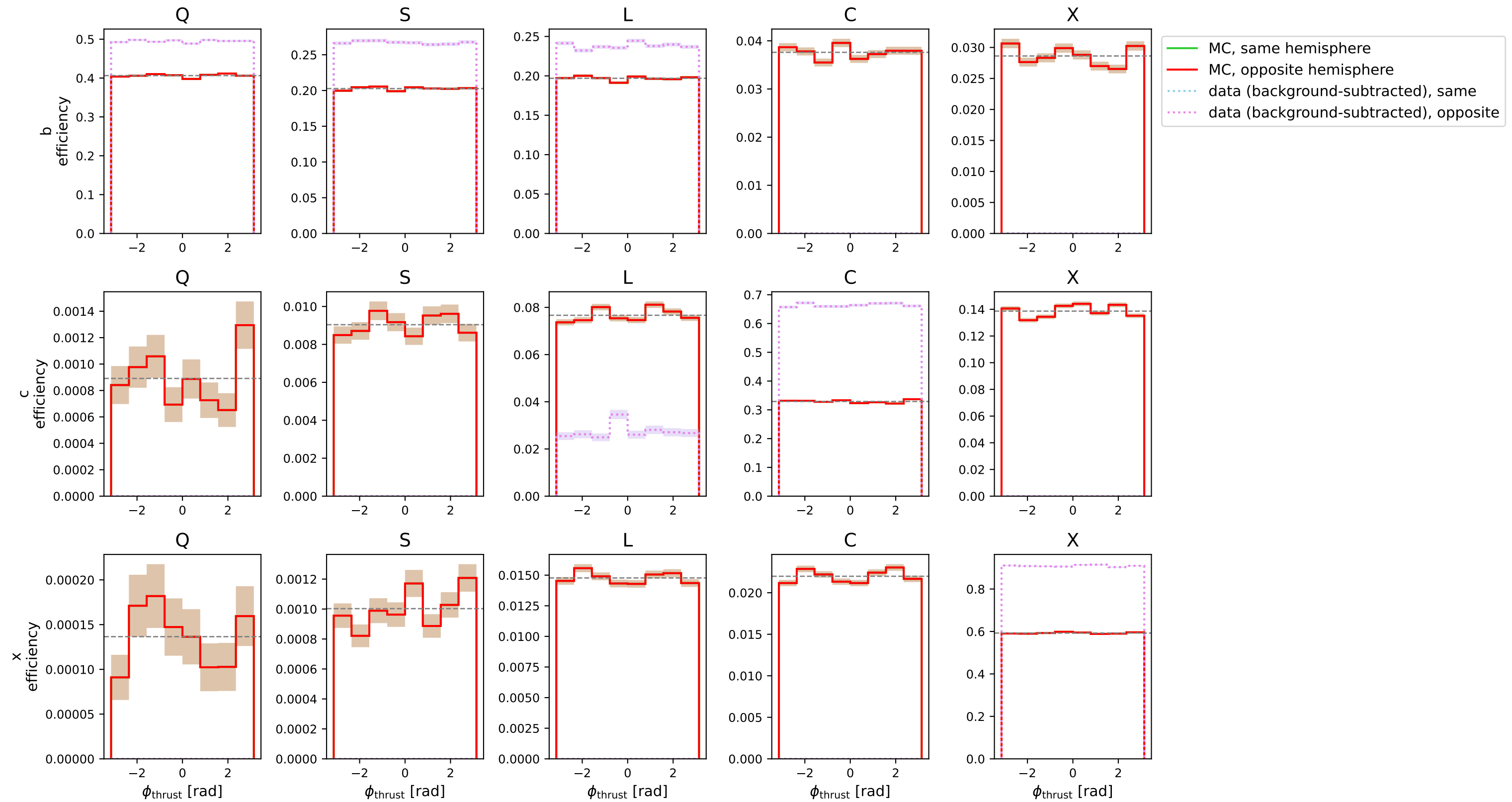
Same vs. opposite hemisphere efficiency vs. \phi_{\text{thrust}}
