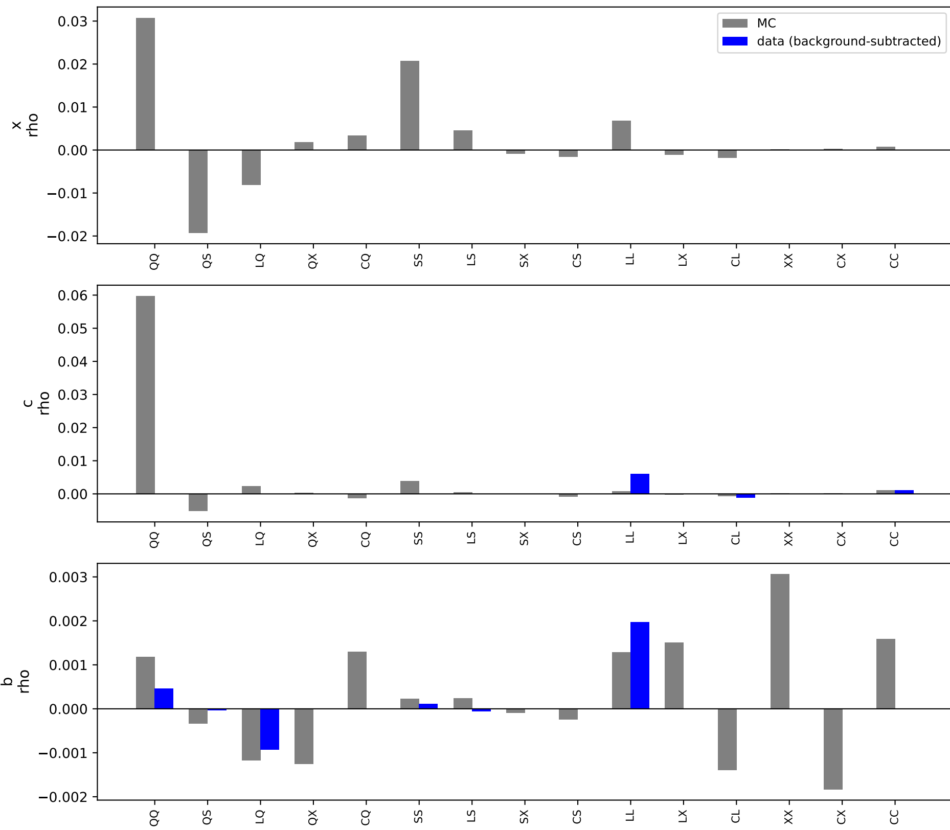
Aggregate correlation per tag pair, variable: cos_theta_thrust
