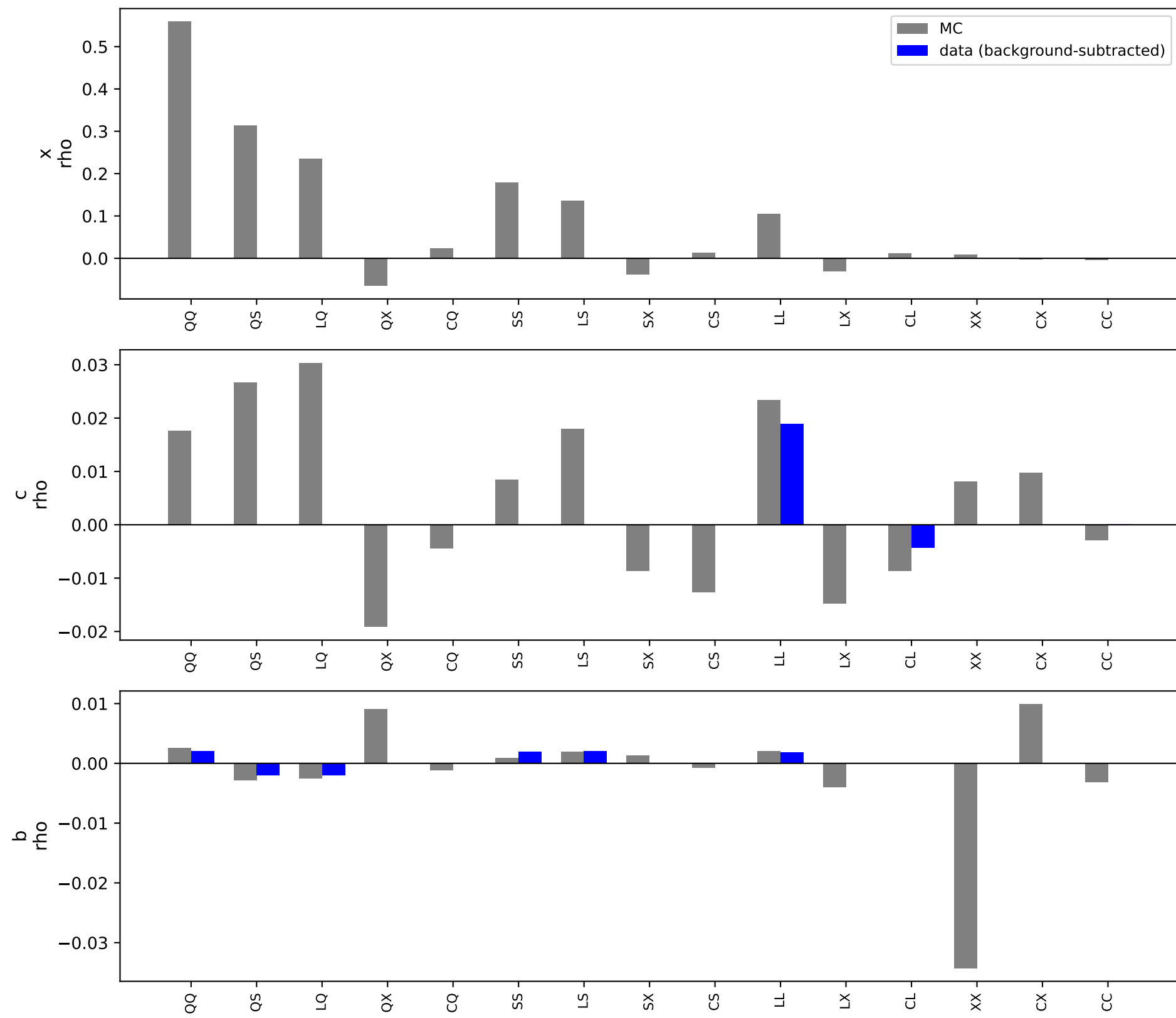
Aggregate correlation per tag pair, variable: jet_momentum
