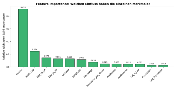
Figure 3. Featureimportance
