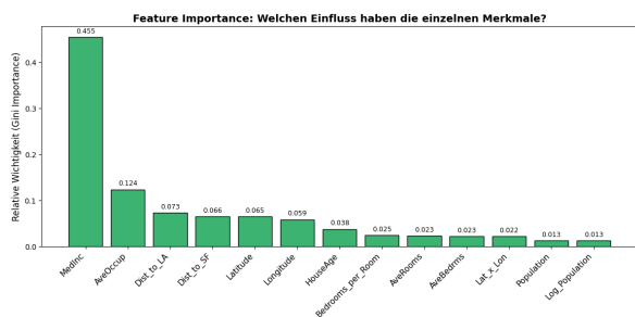
Figure 3. Featureimportance
