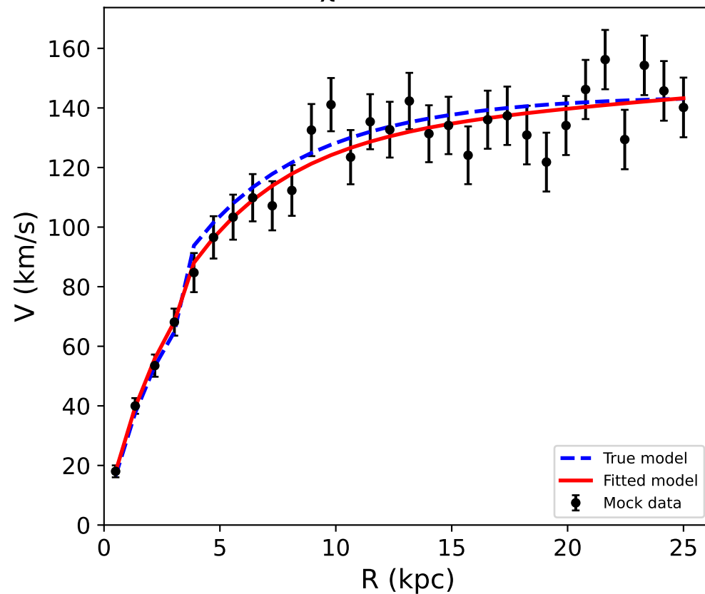
Mock_Massive_4 \chi^2/\text{dof} = 0.77
