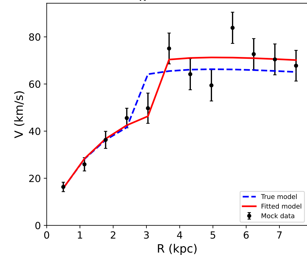
Mock_HSB_5 \chi^2/\text{dof} = 1.29
