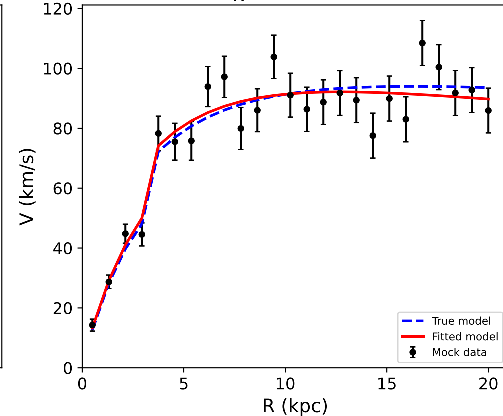
Mock_Spiral_3 \chi^2/\text{dof} = 1.32
