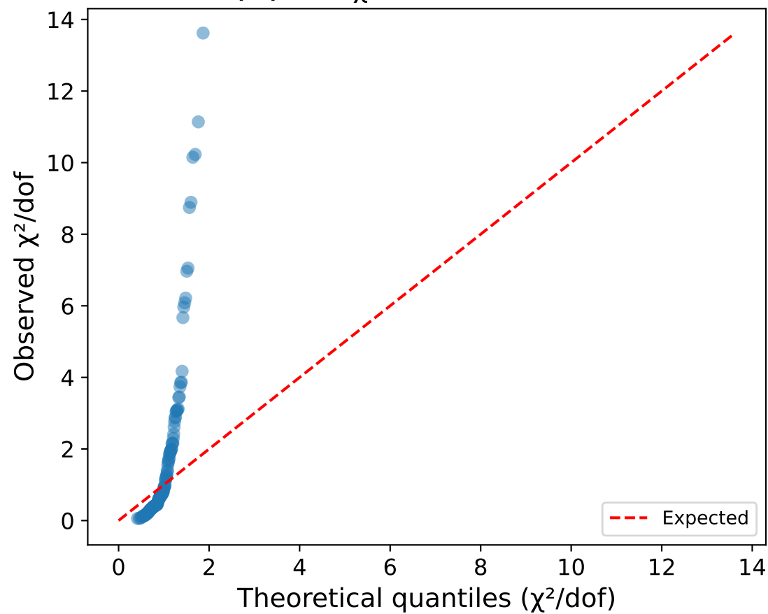
Q-Q Plot: \chi^2 Distribution Check
