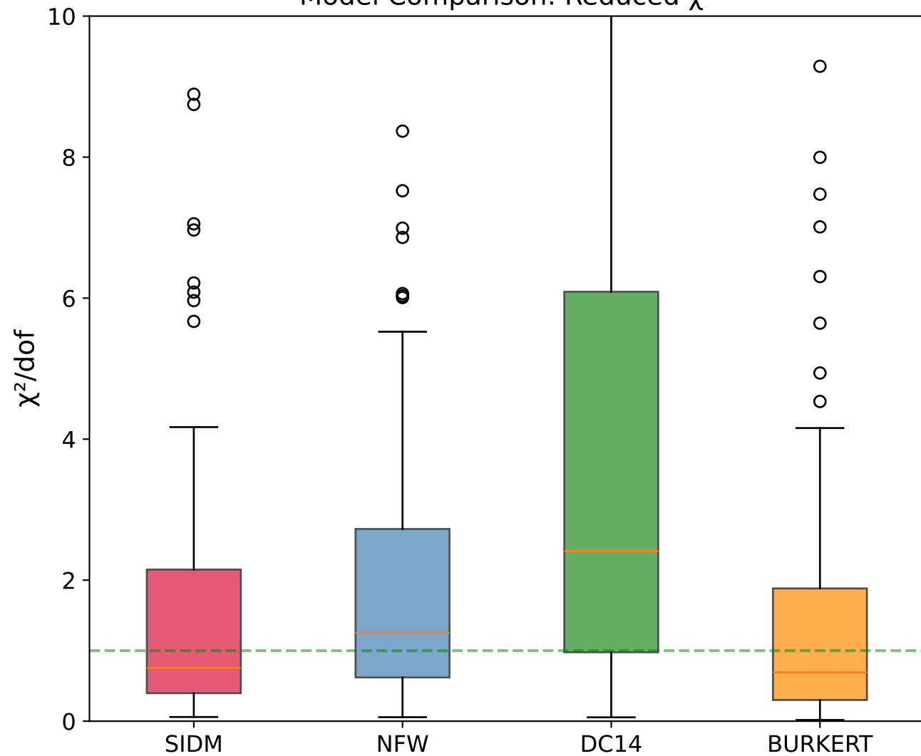
Model Comparison: Reduced \chi^2
