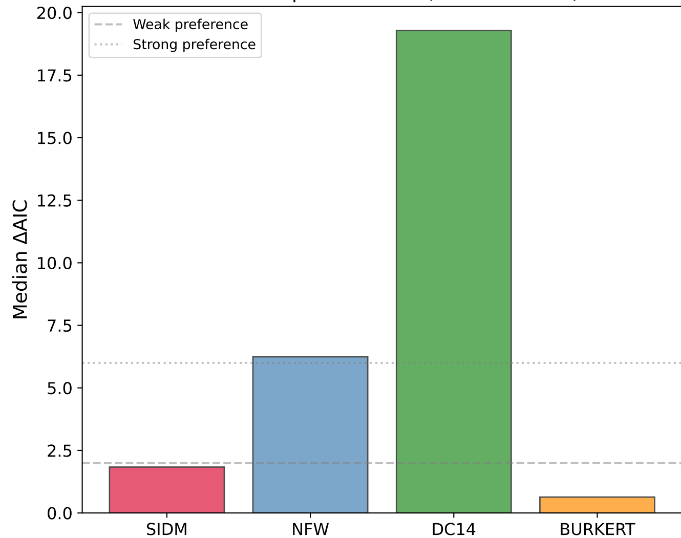
Model Comparison: \Delta\text{AIC} (lower is better)
