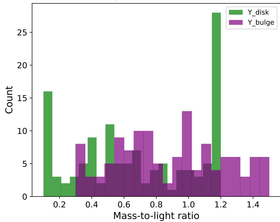
M/L ratio distribution
