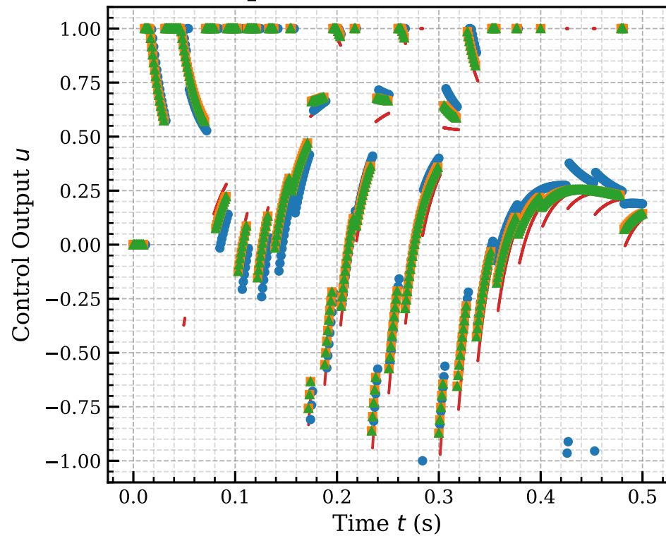
pid.u - dt = 0.001 s
