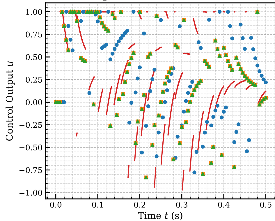
pid.u - dt = 0.005 s
