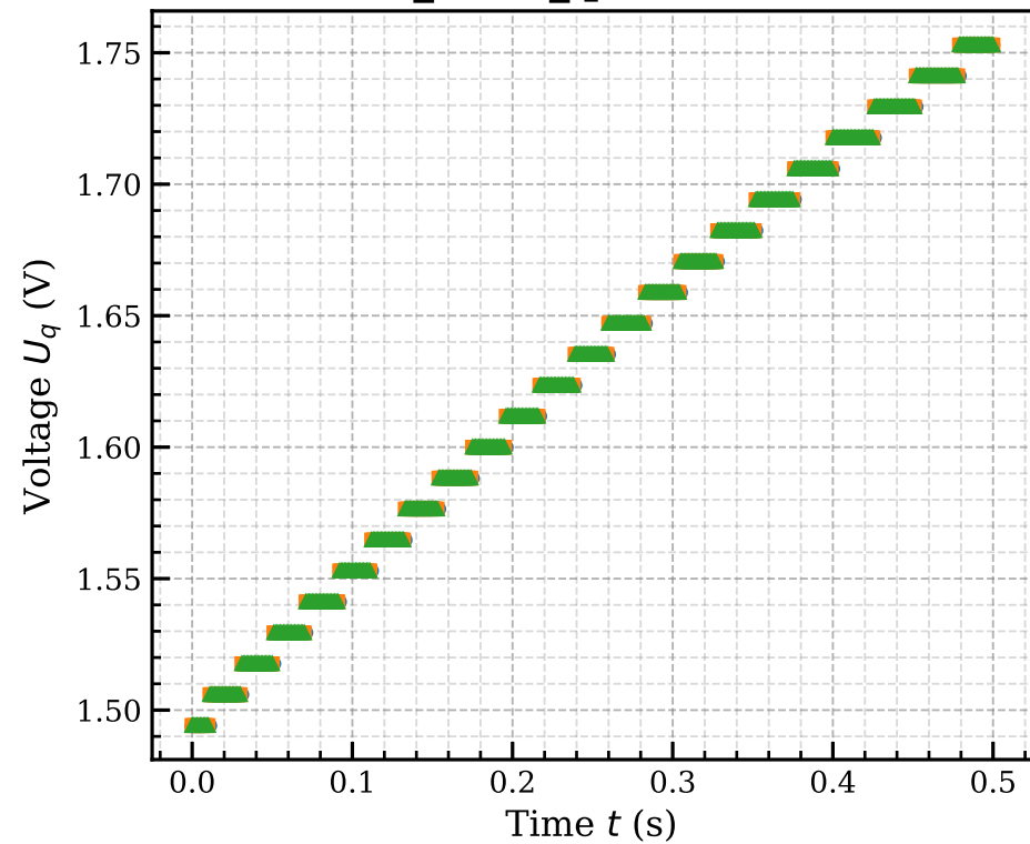
sensor_ref.U_q - dt = 0.001 s
