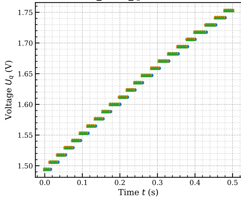
sensor_ref.U_q - dt = 0.005 s
