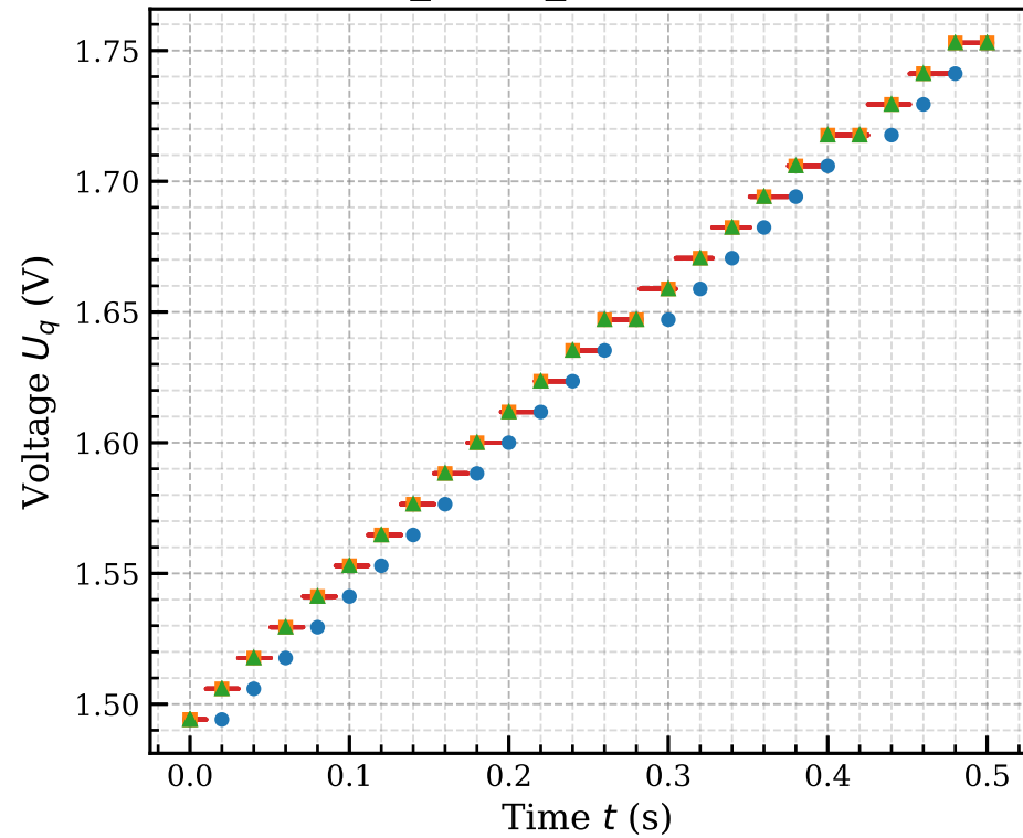
sensor_ref.U_q - dt = 0.020 s
