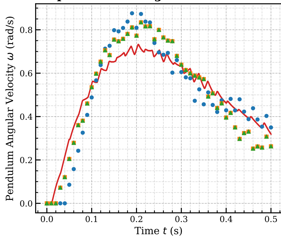
pendulum.omega - dt = 0.010 s
