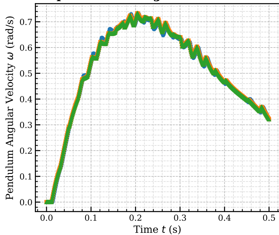
pendulum.omega - dt = 0.001 s
