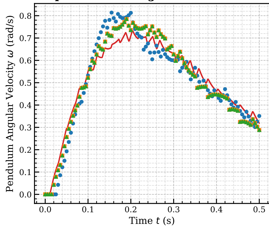
pendulum.omega - dt = 0.005 s
