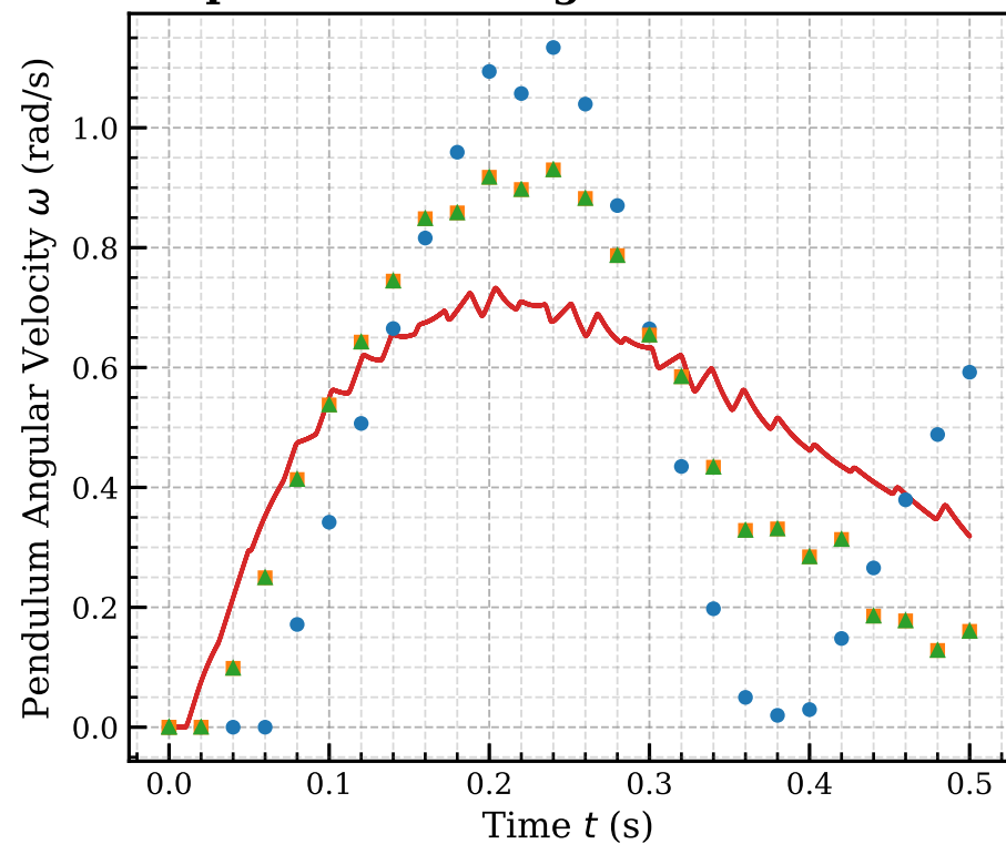
pendulum.omega - dt = 0.020 s
