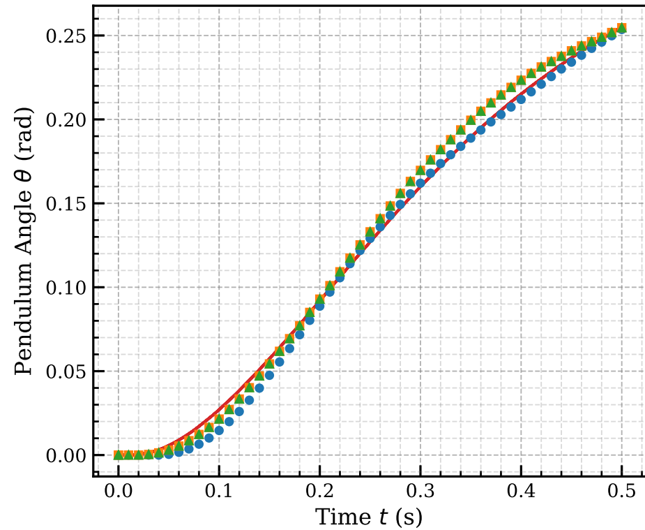
pendulum.q - dt = 0.010 s
