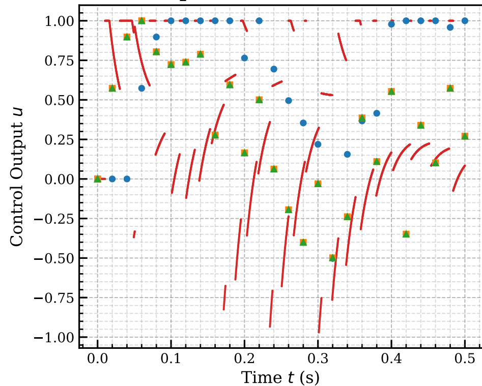
pid.u - dt = 0.020 s
