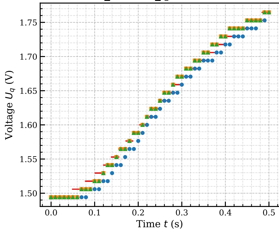
sensor_state.U_q - dt = 0.010 s
