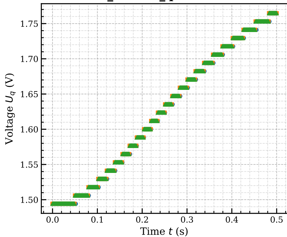
sensor_state.U_q - dt = 0.001 s
