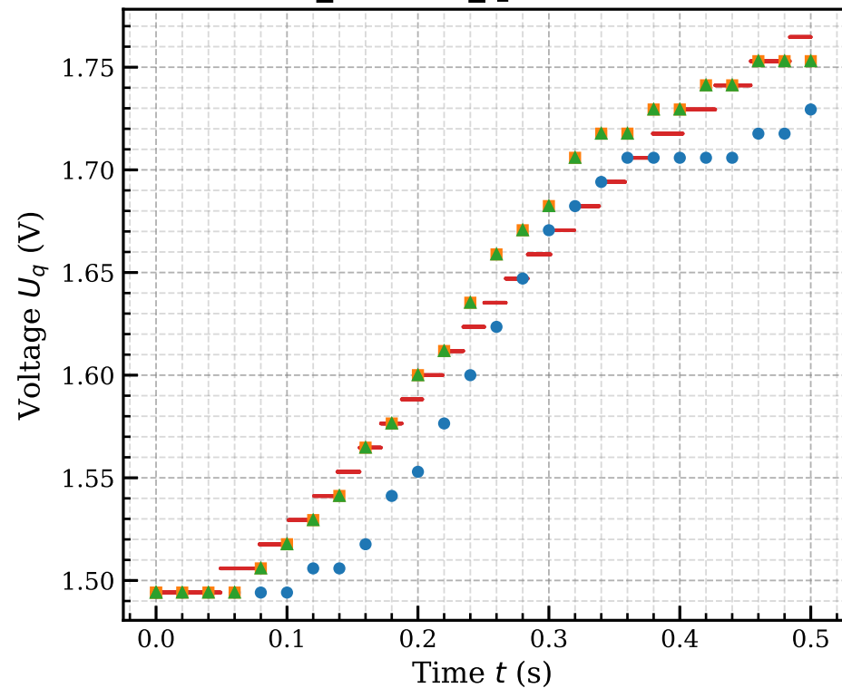
sensor_state.U_q - dt = 0.020 s
