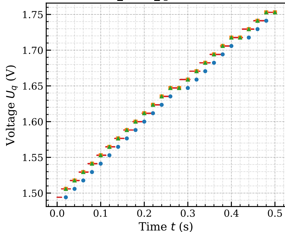
sensor_ref.U_q - dt = 0.020 s
