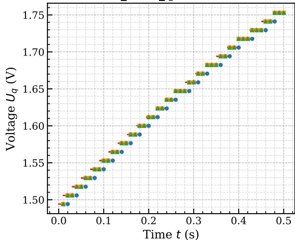
sensor_ref.U_q - dt = 0.010 s
