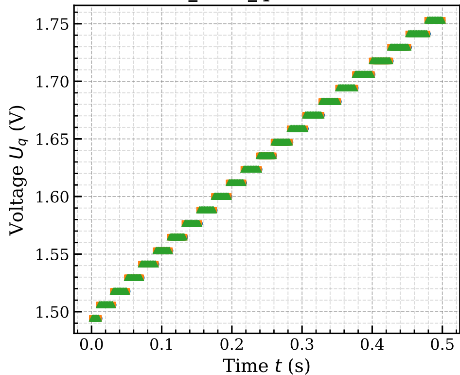
sensor_ref.U_q - dt = 0.001 s
