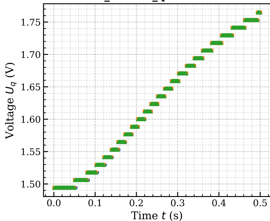
sensor_state.U_q - dt = 0.001 s
