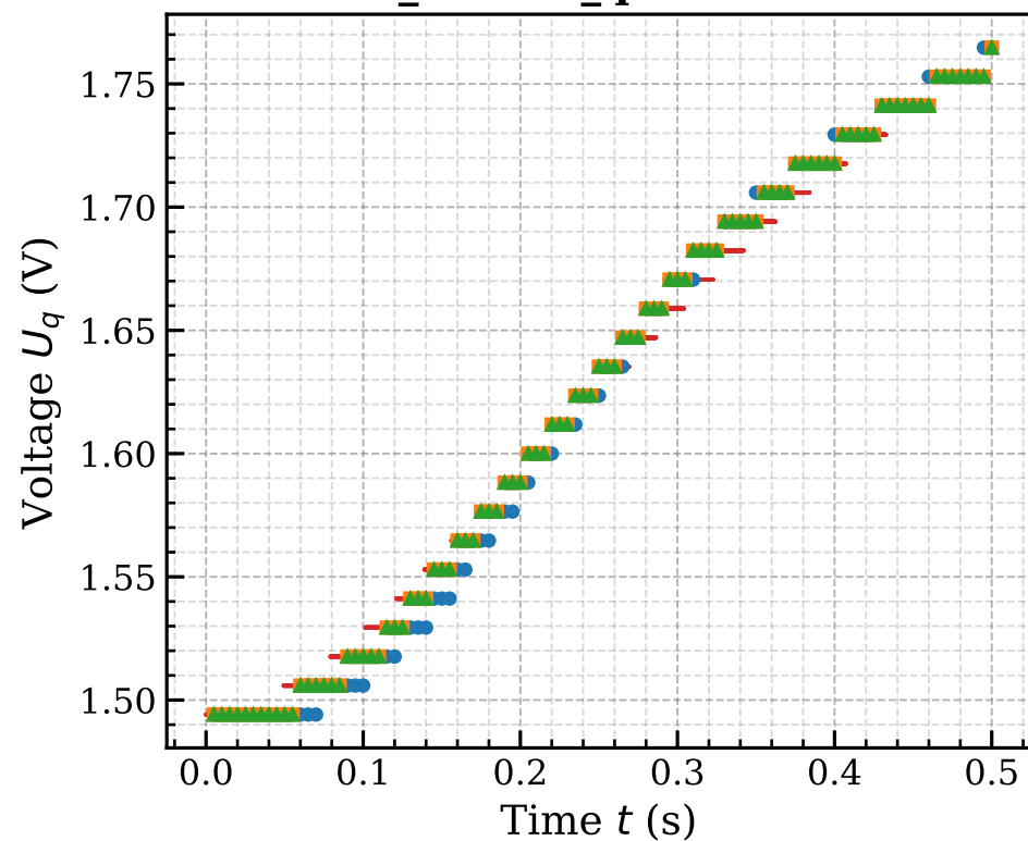
sensor_state.U_q - dt = 0.005 s
