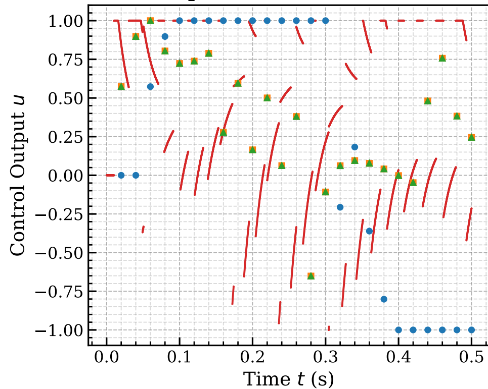
pid.u - dt = 0.005 s
