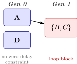
(c) Condensed graph
