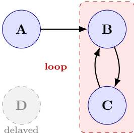
(b) Zero-delay graph
