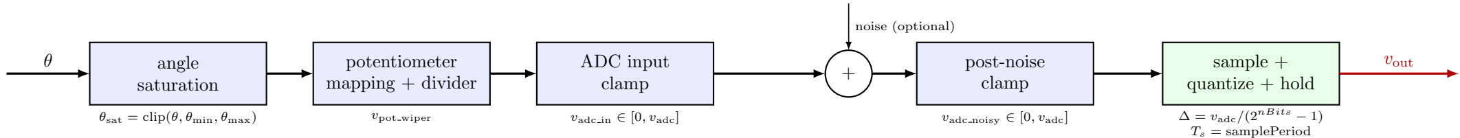
AngleSensor measurement chain (ADC model)
