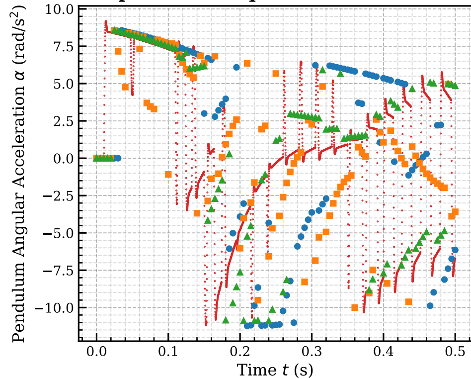
pendulum.alpha - dt = 0.005 s
