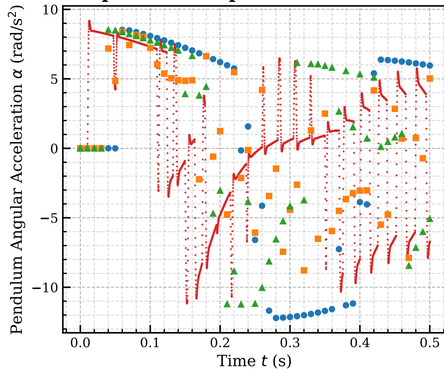
pendulum.alpha - dt = 0.010 s
