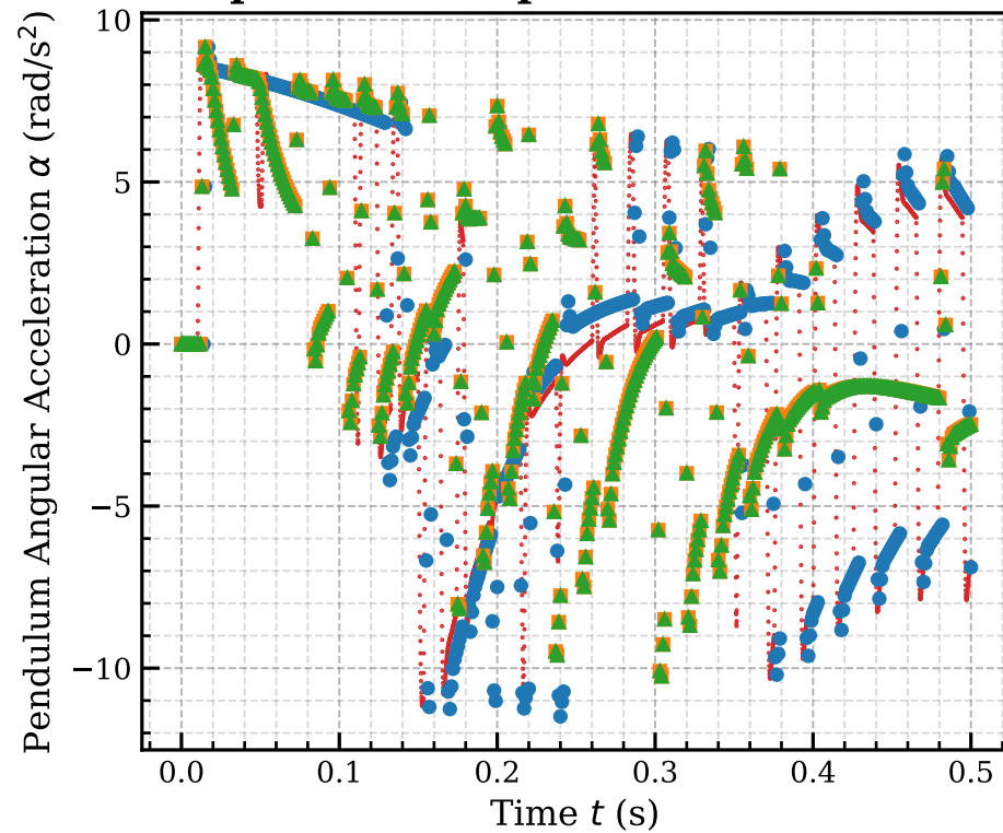
pendulum.alpha - dt = 0.001 s
