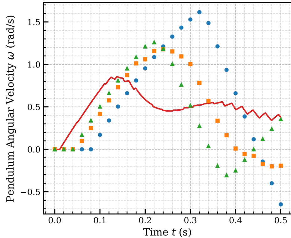
pendulum.omega - dt = 0.020 s
