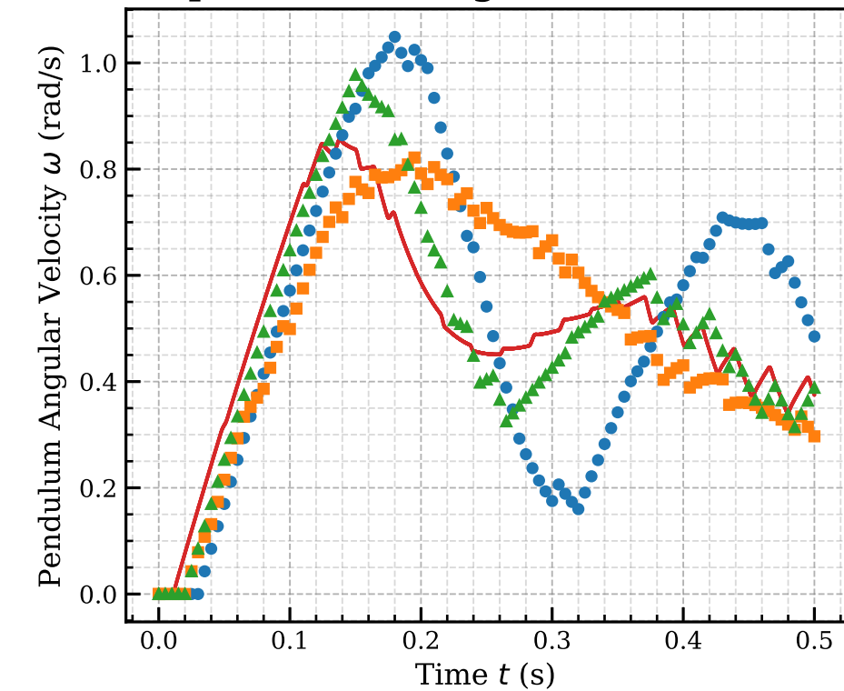
pendulum.omega - dt = 0.005 s
