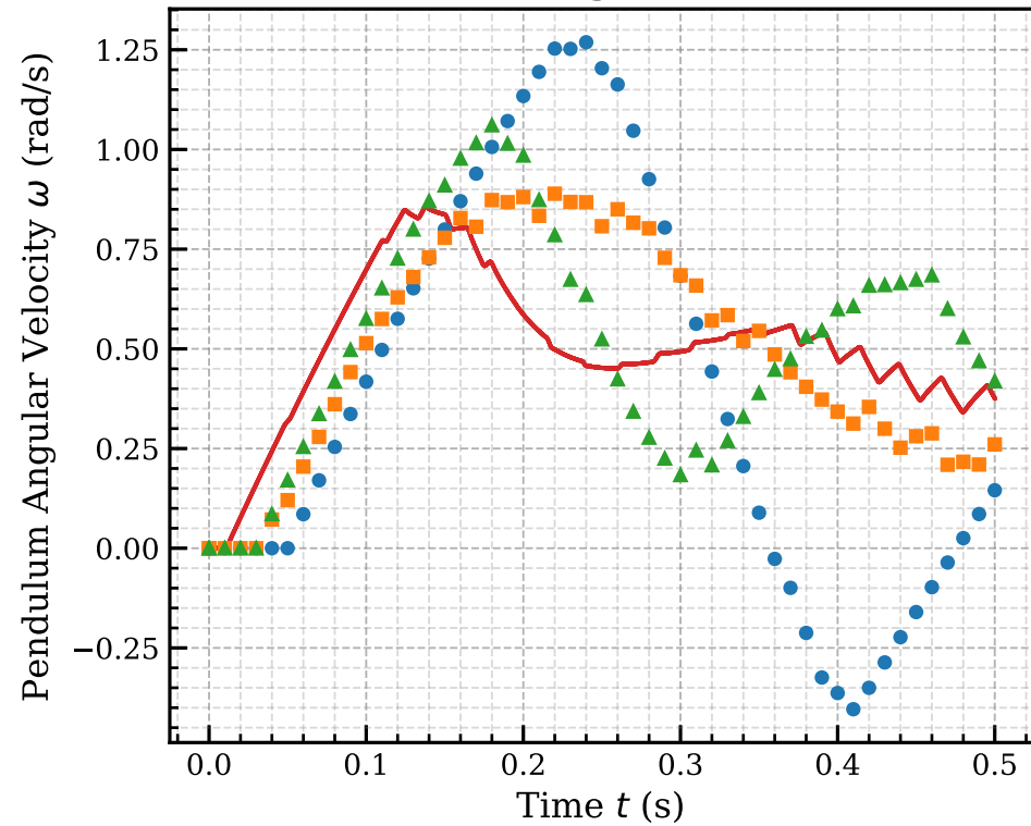
pendulum.omega - dt = 0.010 s
