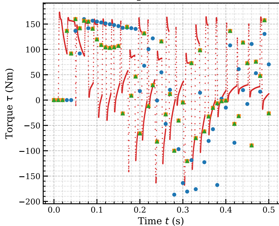
drive.torque - dt = 0.010 s
