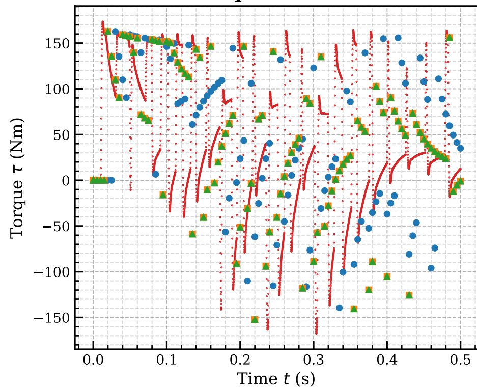
drive.torque - dt = 0.005 s
