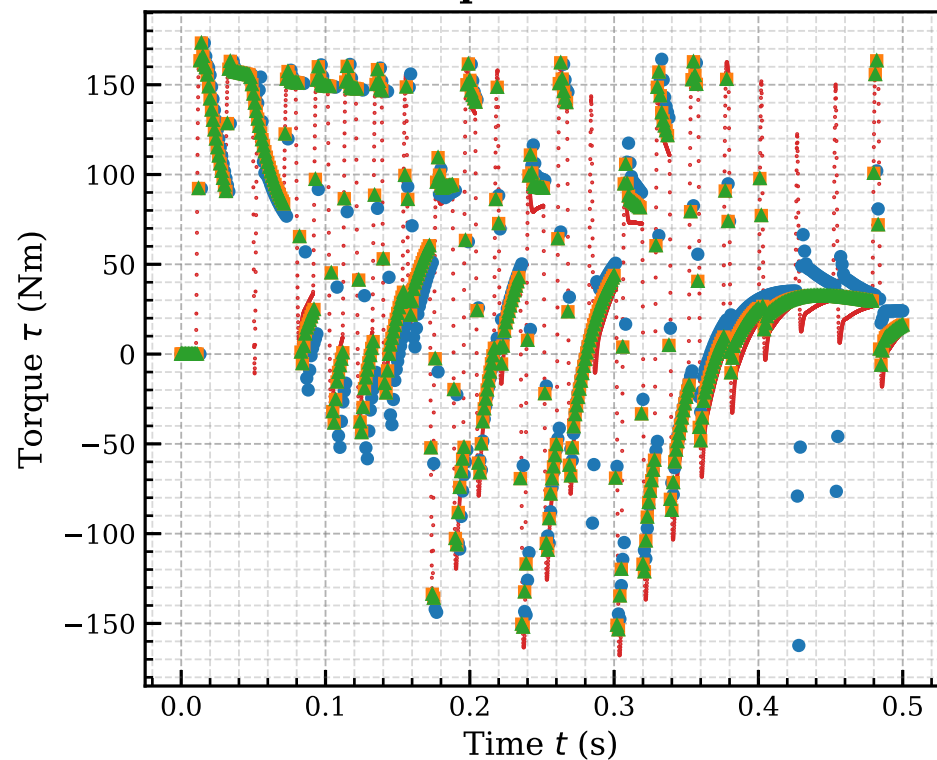
drive.torque - dt = 0.001 s
