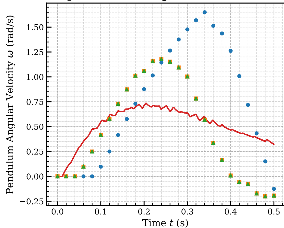
pendulum.omega - dt = 0.020 s
