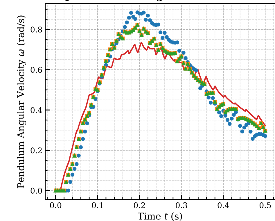
pendulum.omega - dt = 0.005 s
