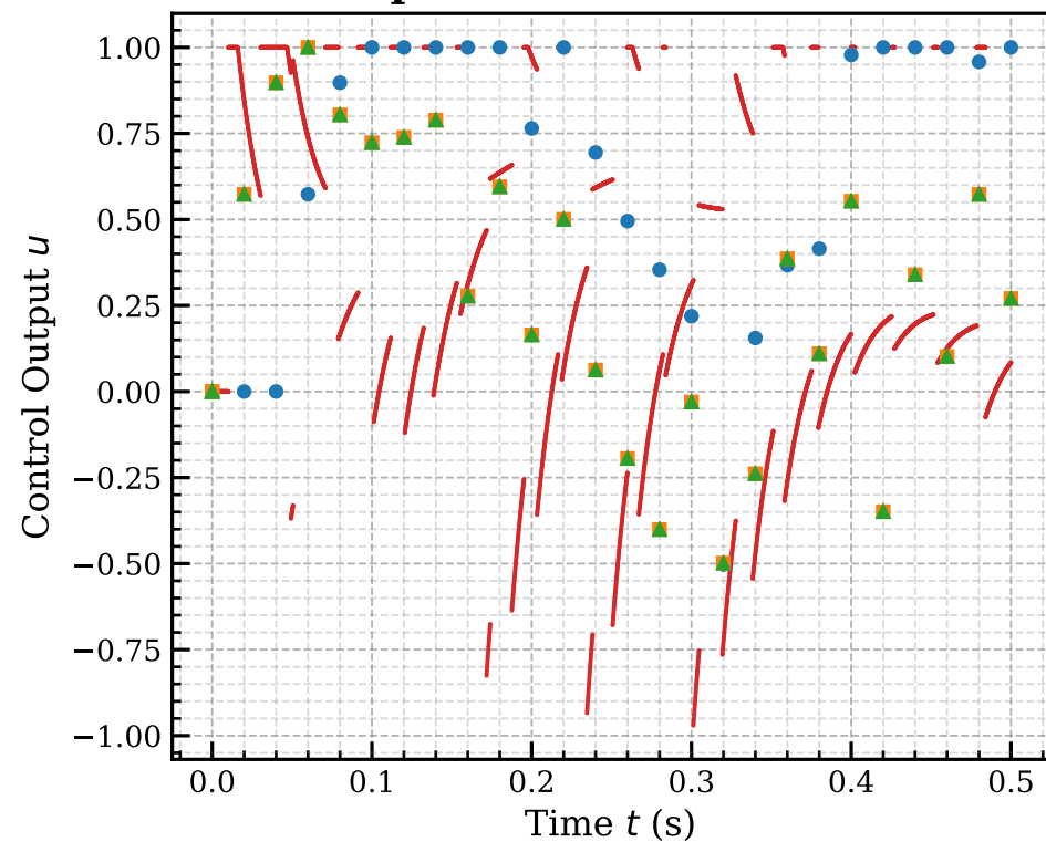
pid.u - dt = 0.020 s
