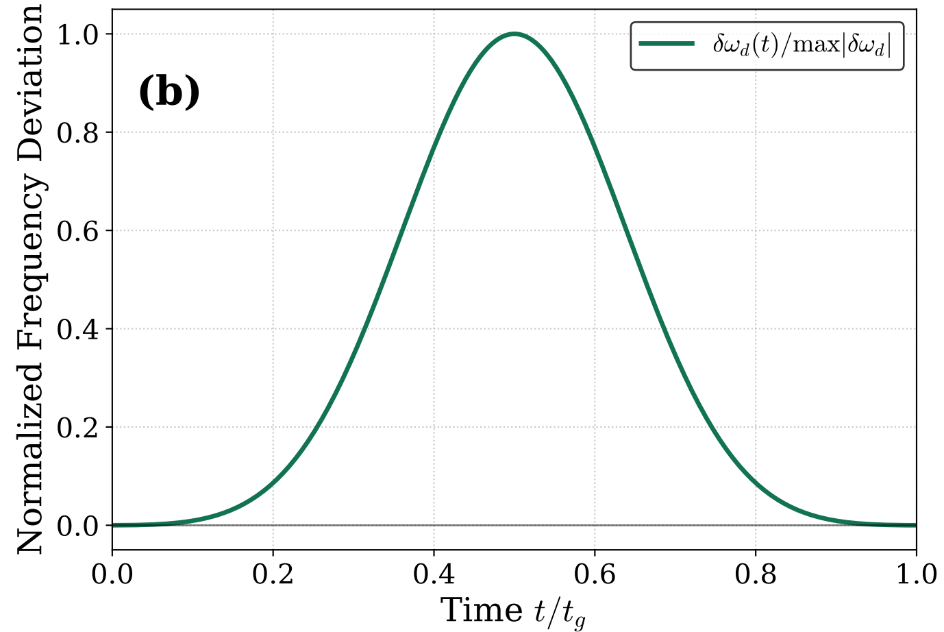
Gaussian Dynamic Shift ( \sigma_r = 0.2 )
