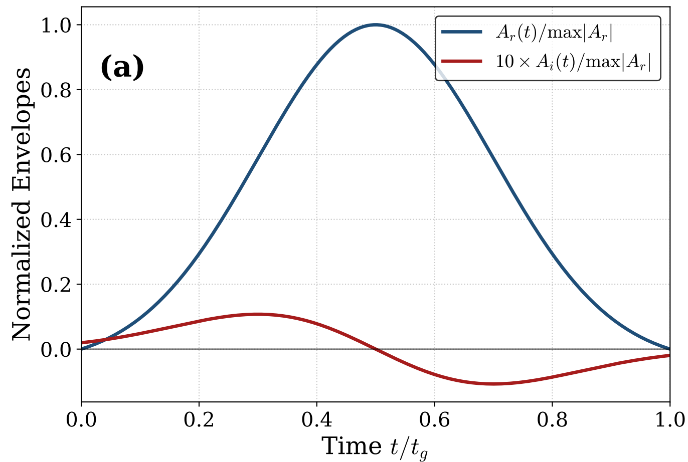
Gaussian DRAG Envelope ( \sigma_r = 0.2 )
