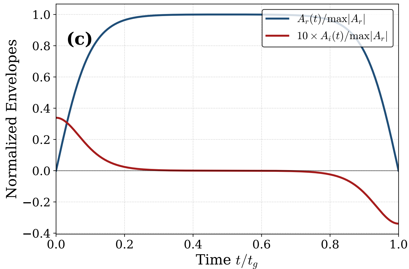
Tanh DRAG Envelope ( \sigma_r = 0.1 )
