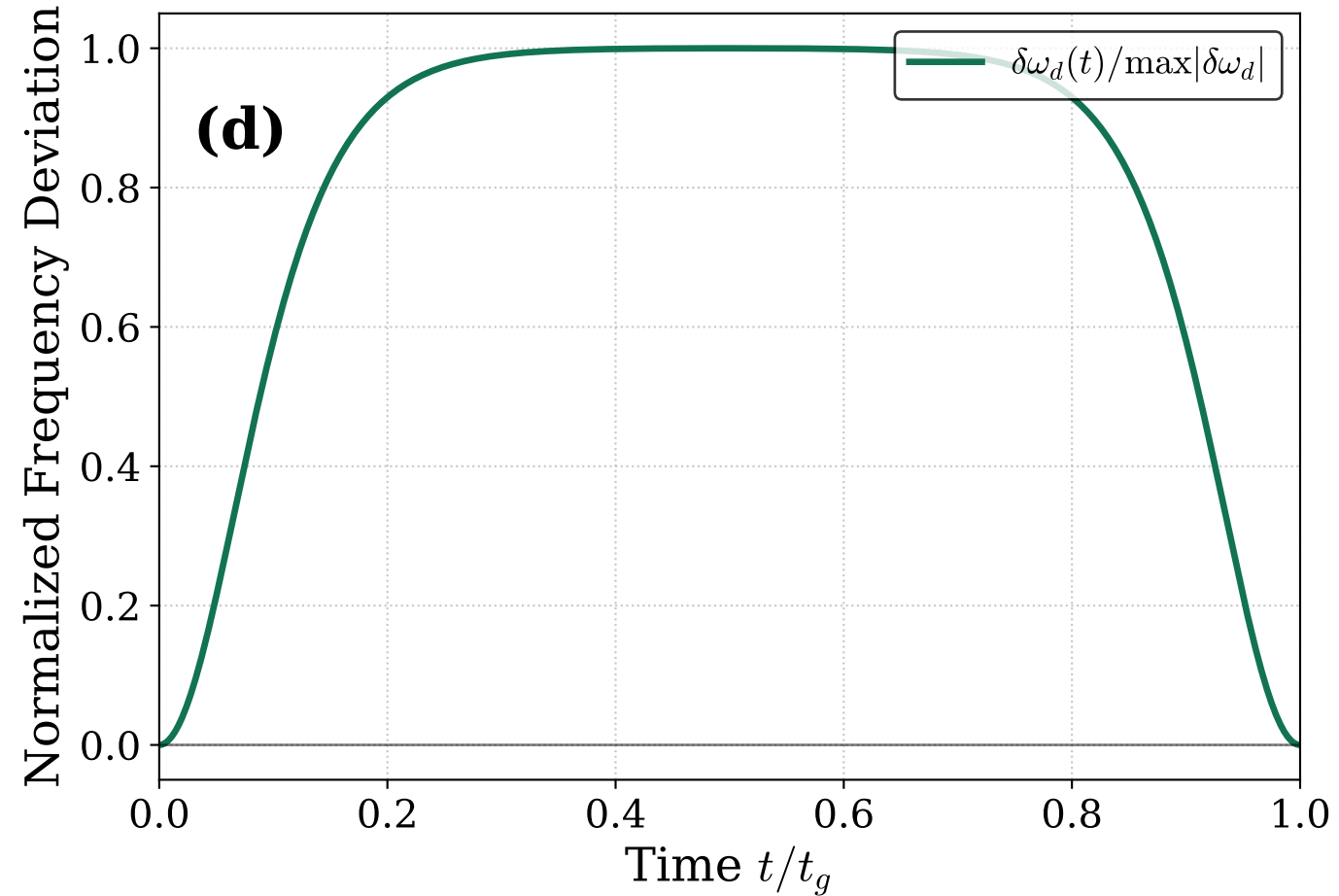
Tanh Dynamic Shift ( \sigma_r = 0.1 )
