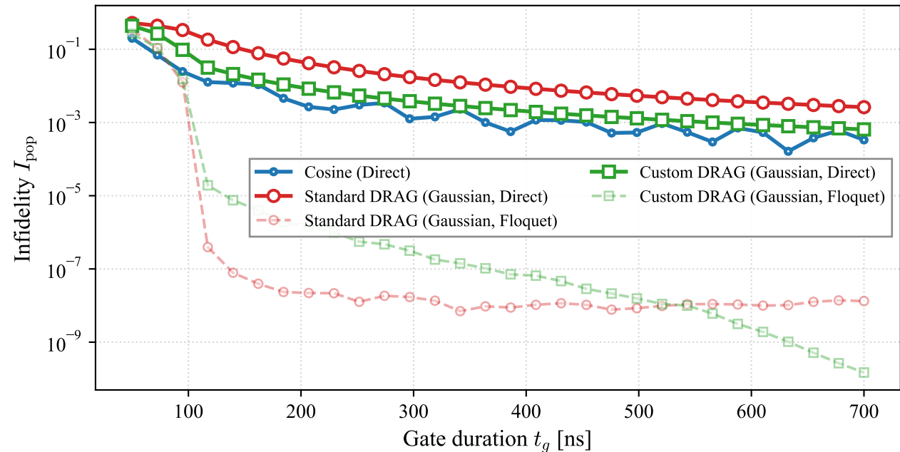
Gaussian Pulse: Population Infidelity Comparison
