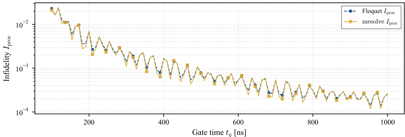
(c) Gate Time Correction: Process Infidelity
