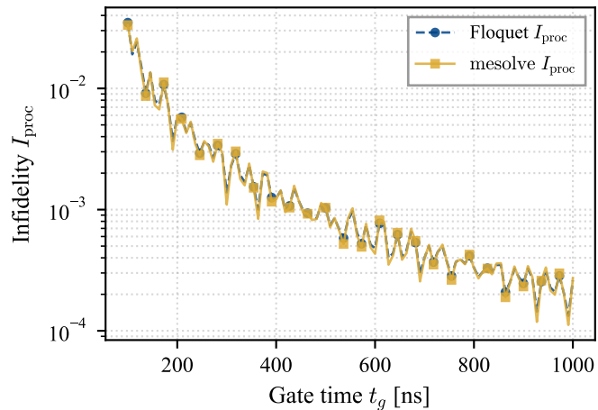
(c) Gate Time Correction: Process Infidelity
