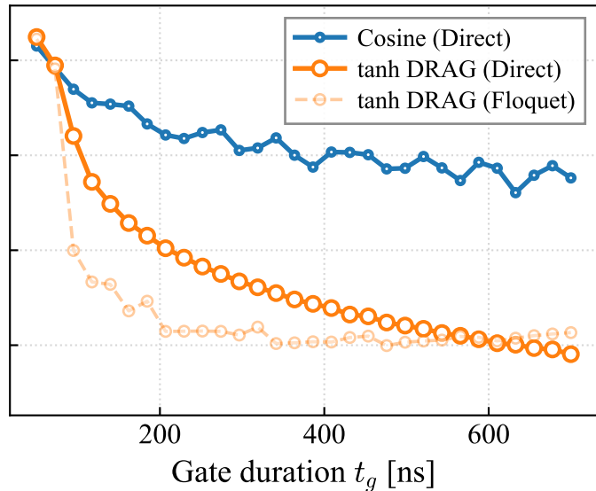
(b) tanh Pulse (FAPT)
