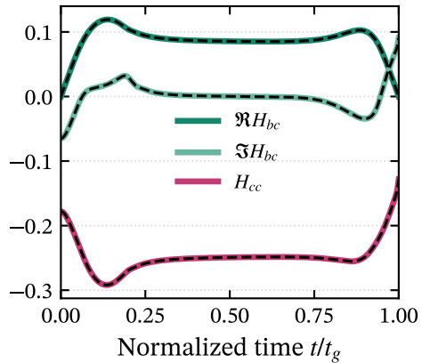
(c) Entries determined by \lambda and \Delta
