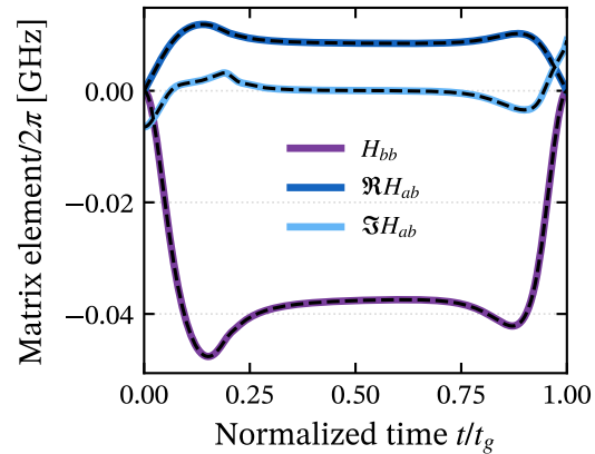
(a) Directly constrained entries
