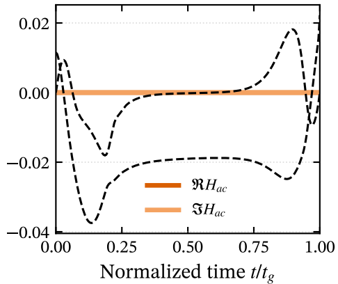
(b) Second-harmonic contribution
