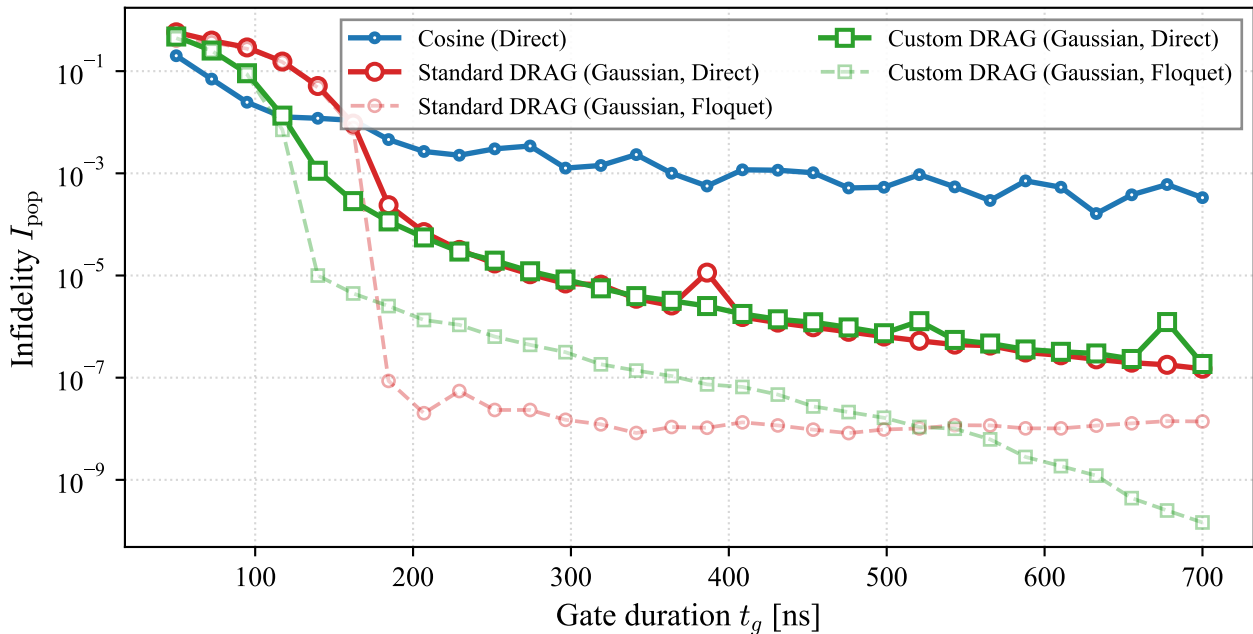
Gaussian Pulse (FAPT): Population Infidelity Comparison
