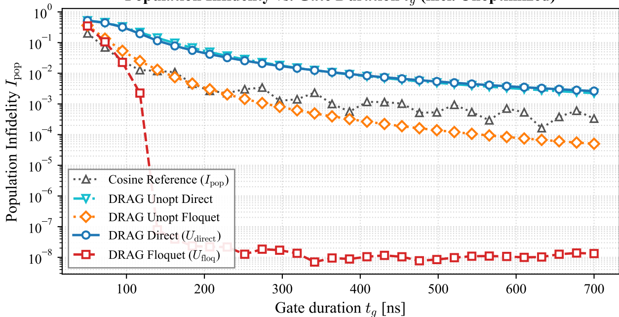
Population Infidelity vs. Gate Duration t_g (incl. Unoptimized)
