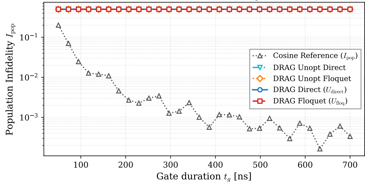
Population Infidelity vs. Gate Duration t_g (incl. Unoptimized)
