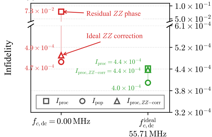
(c) Verification of the ZZ correction
