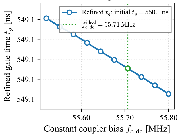
(b) Gate-time refinement enforcing \theta_1 = \theta_2
