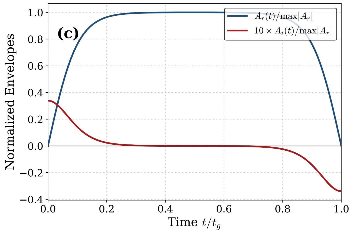
Tanh DRAG Envelope ( \sigma_r = 0.1 )
