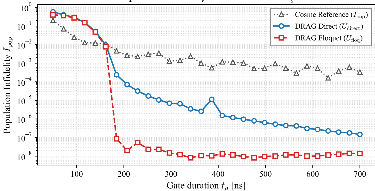
Population Infidelity vs. Gate Duration t_g
