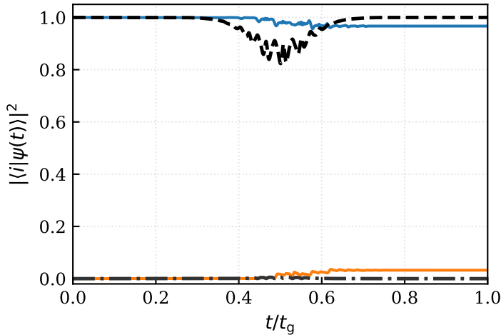
(a) FPT without FAPT corrections
