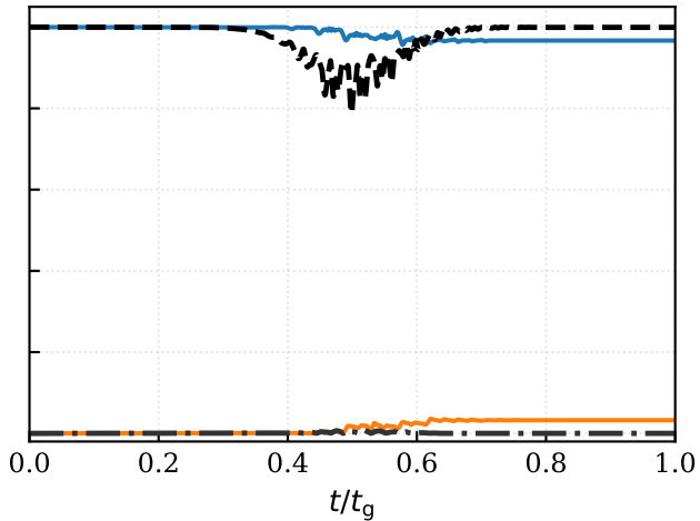
(b) Complete FAPT prediction
