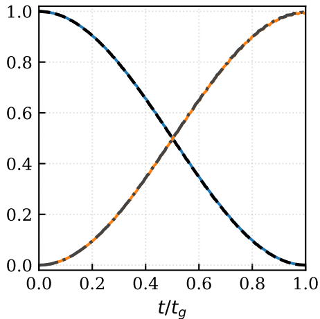
(a) Cosine
