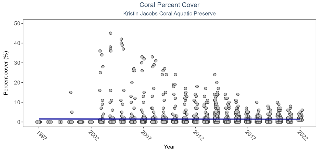
Figure 4: Scatter plot of live coral coverage over time as a percent of reef surface. Species groups include octocorals, milleporans, and scleractinians. If the time series included five or more years of observations, a significant (blue) or non-significant (magenta) trend line is also shown. Data points are jittered horizontally to reduce overlap.
