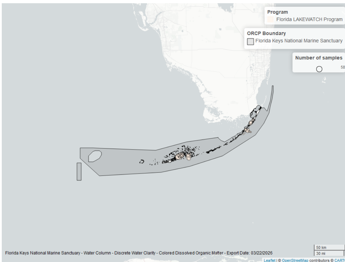
Figure 53: Map showing location of discrete water quality sampling locations within the boundaries of Florida Keys National Marine Sanctuary . The bubble size on the maps above reflect the amount of data available at each sampling site.
